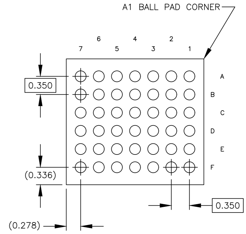
BOTTOM VIEW 42 BUMPS
