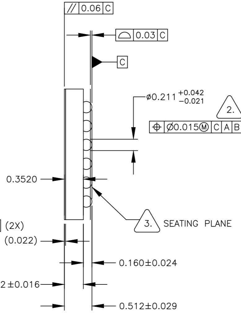
SIDE VIEW
